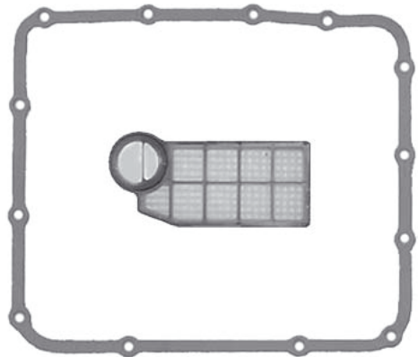
ZF 4HP14 VOLVO & MG Pan Gasket Special Order Filter 4HP14.FIL01
