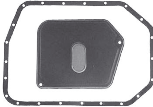
ZF 5HP24 BMW, JAGUAR, LANDROVER Pan Gasket 5HP24.GAS01 Filter 5HP24.FIL01 Filter Pick up 5mm
