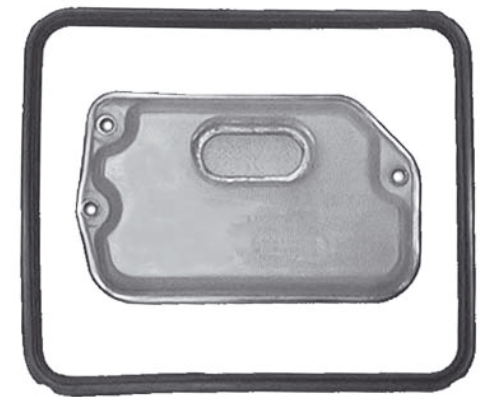
ZF 4HP18FLA/FLE Pan Gasket 4HP18.GAS08 Filter 4HP18.FIL02
