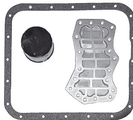
SUBARU 4 SPEED 1999-ON Pan Gasket SUB4.GAS11 Internal Filter SUB4.FIL04 External Filter SUB4.FIL05
