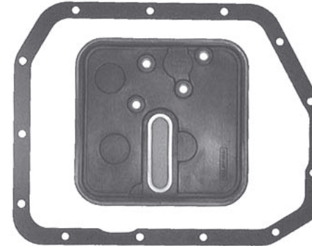
HYUNDAI A4BF-1 Pan Gasket KM177.GAS06 Filter KM177.FIL01
