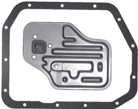
HYUNDAI A4BF-1 Pan Gasket KM177.GAS06 Filter KM170.FIL05
