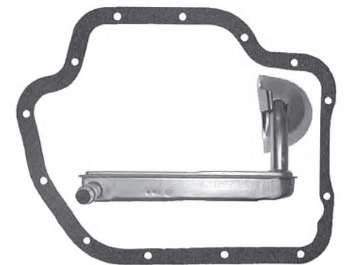
TH400 Pan Gasket TH400.GAS01 Filter TH400.FIL03 1964-1967
