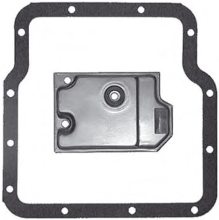
TRIMATIC/TH180 Pan Gasket TH180.GAS01 Filter TH180.FIL01
